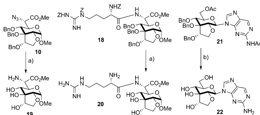
Scheme 6. Debenzylation attempts on model compounds. a) H 2 (30 psi), 10 % Pd/C, glacial AcOH, 2.5 h; b) H 2 (400 psi), 10 % Pd/C, glacial AcOH, 8 h then NH 4 OH/MeOH 1:1, 60 °C, 24 h, 86 %.
