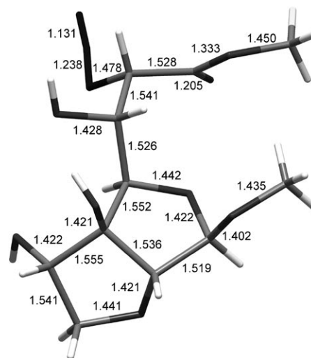
Figure 1. X-ray structure of the fused tetrahydrofuran derivative A .
