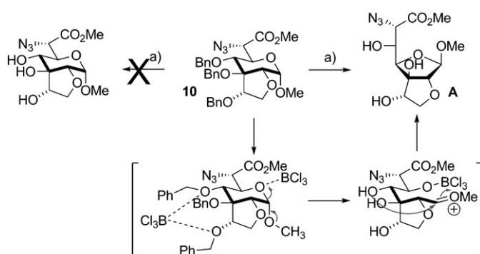
Scheme 3. Proposed mechanism for the skeleton rearrangement of azidoester 10 . a) BCl 3 (1 M in CH 2 Cl 2 ), CH 2 Cl 2 , -78 to 0 °C, 65 %.
