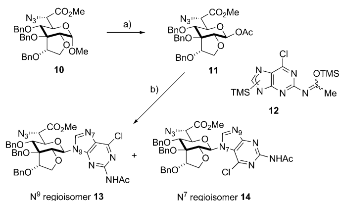
Scheme 4. N-glycosylation step. a) Ac 2 O, H 2 SO 4 5 % in AcOH, -20 to 0 °C, 39 %; b) 12 , TMSOTf, solvent and temperature (see Table 1).
