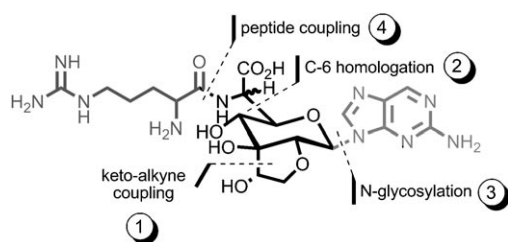
Scheme 1. Key disconnections planned for the synthesis of the miharamycin B framework.
