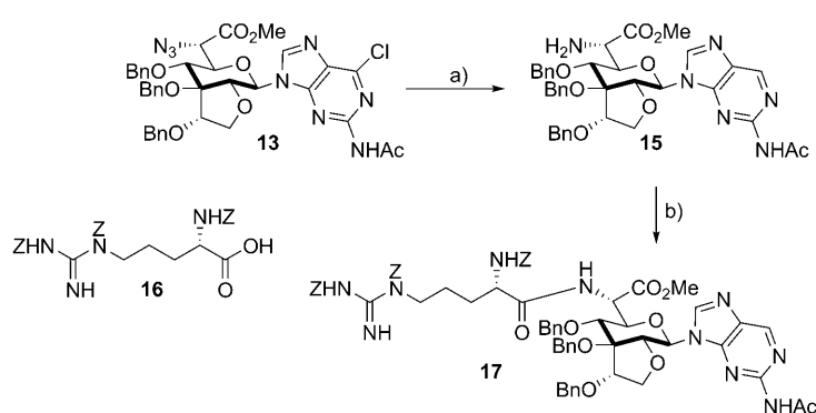
Scheme 5. Synthesis of the skeleton of miharamycin B. a) H 2 , 10 % Pd/C, Et 3 N, EtOAc; b) 16 , isobutyl chloroformate, Et 3 N, THF, −20 °C, 70 % over 2 steps.
