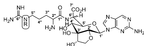
miharamycin A (1): R = OH miharamycin B (2): R = H
