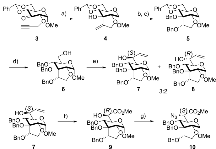
Scheme 2. Synthesis of azido ester 10 . a) \text{SmI}_2 (0.1 M in THF), HMPA, t BuOH, THF, 94%; b) \text{O}_3 , -78^\circ\text{C} , \text{Me}_2\text{S} , \text{CH}_2\text{Cl}_2 then \text{NaBH}_4 , EtOH, 0^\circ\text{C} , 84% over two steps; c) \text{BnBr} , \text{NaH} , DMF, 95%; d) \text{LiAlH}_4/\text{AlCl}_3 , \text{Et}_2\text{O}/\text{CH}_2\text{Cl}_2 2:1, 50^\circ\text{C} , 88%; e) (\text{COCl})_2 , DMSO, \text{Et}_3\text{N} , \text{CH}_2\text{Cl}_2 , -78^\circ\text{C} then \text{CH}_2=\text{CHMgBr} , THF, -78^\circ\text{C} , 65% over 2 steps; f) \text{O}_3 , -78^\circ\text{C} , \text{Me}_2\text{S} , \text{CH}_2\text{Cl}_2 then \text{NaClO}_2 , \text{NaH}_2\text{PO}_4 \cdot \text{H}_2\text{O} , t BuOH/ \text{H}_2\text{O} /2-methyl-but-2-ene 2:2:1 then \text{MeI} , \text{KHCO}_3 , DMF, 65% over three steps; g) \text{TiF}_4 , pyridine, \text{CH}_2\text{Cl}_2 , -78^\circ\text{C} then \text{NaN}_3 , DMF, 82% over 2 steps.
